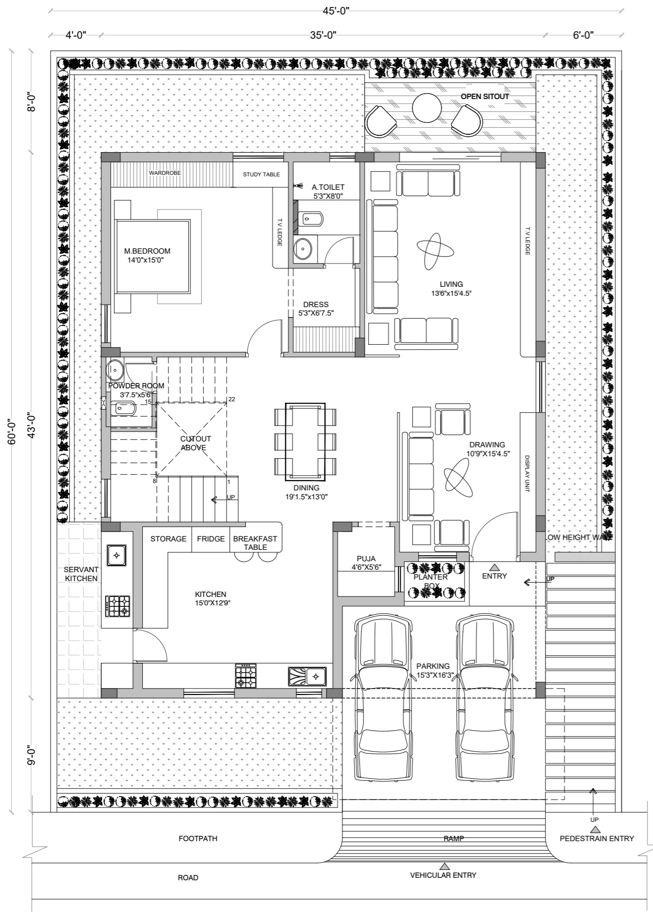
GROUND FLOOR
